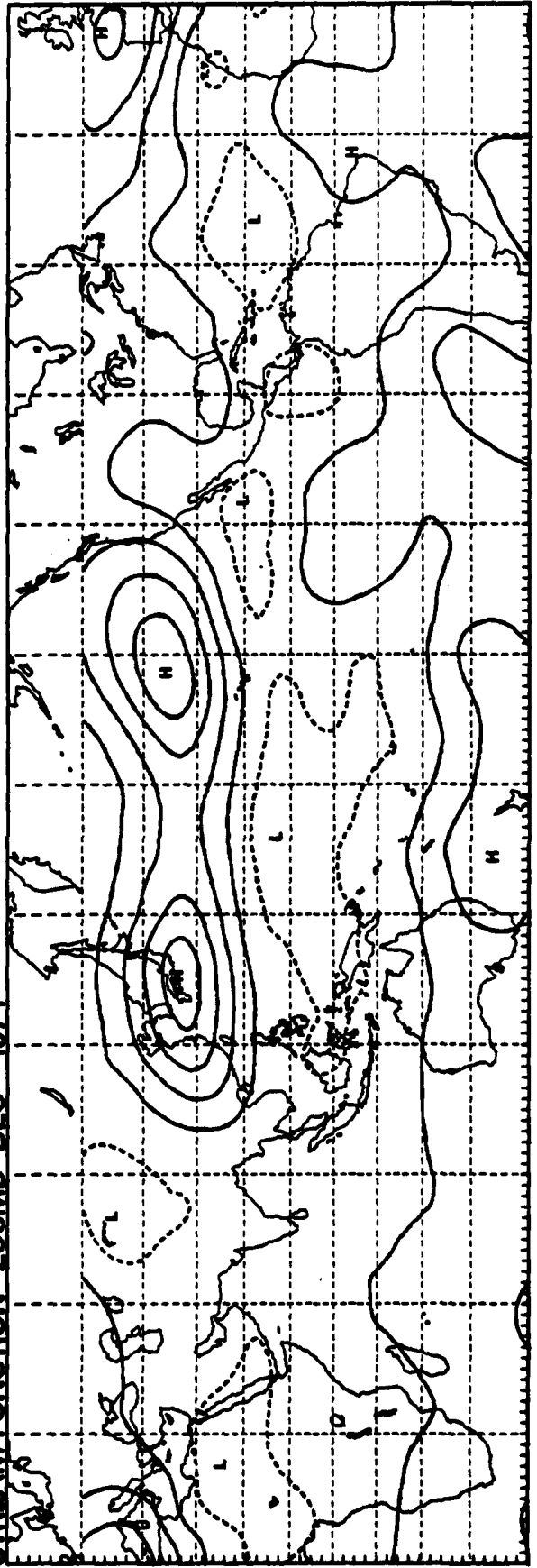
STREAM FUNCTION 200MB DEC 1974
